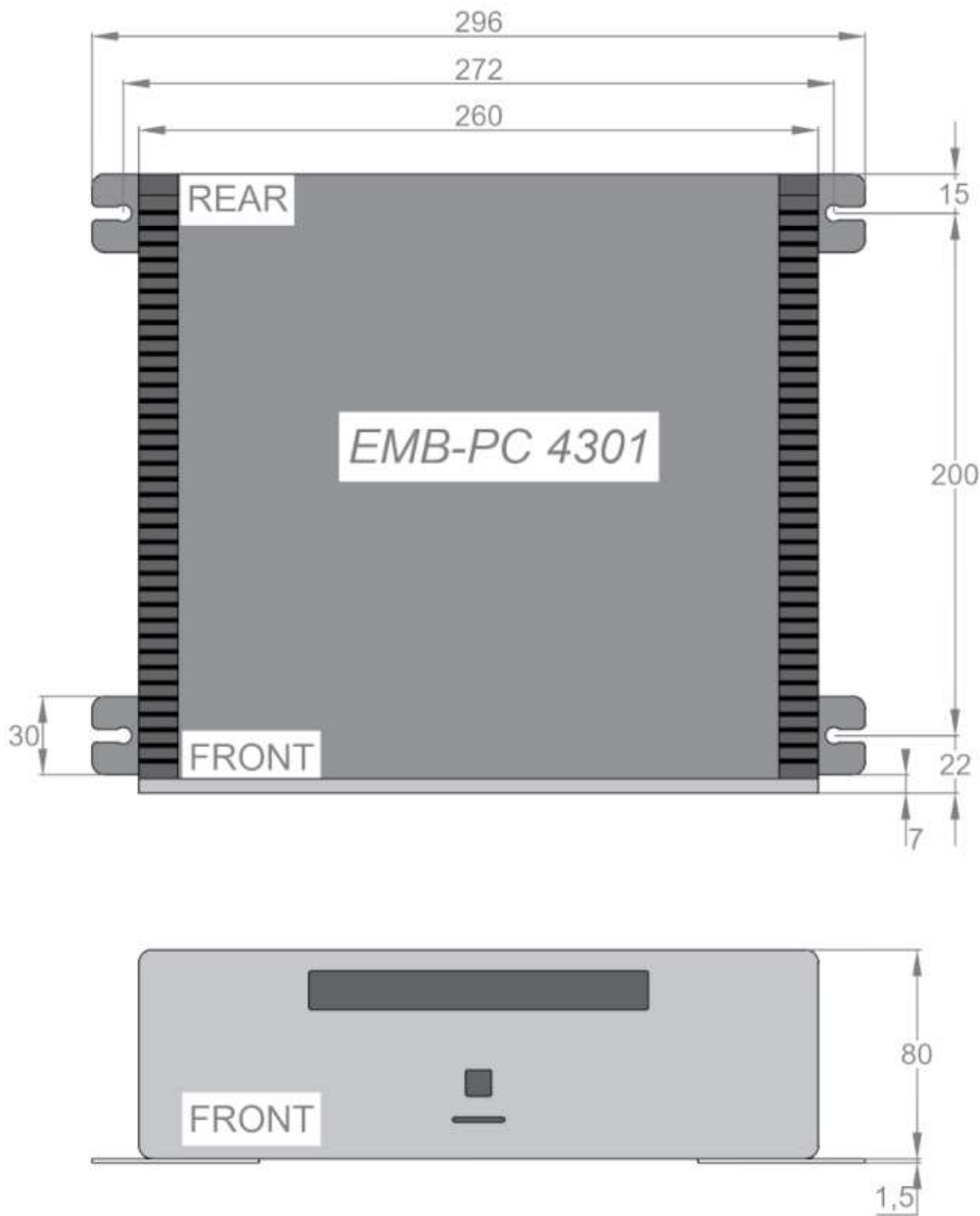
Mechanical Drawings (Unit=mm)
